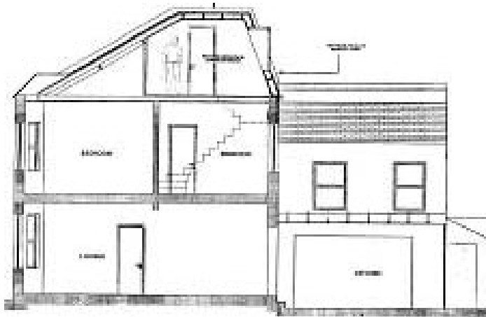
Typical Cross Section of Proposed Extension
